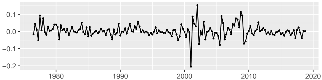
Residuals from ARIMA(3,0,0)(1,0,1)[4] with zero mean
